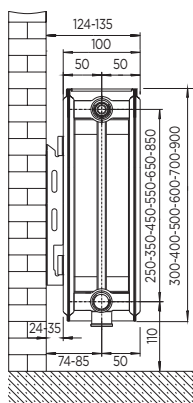
DS Double Panel Double Convactor
