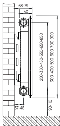
SF Single Panel Single Convactor
