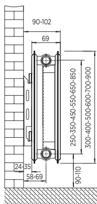
HF Double Panel Single Convactor
