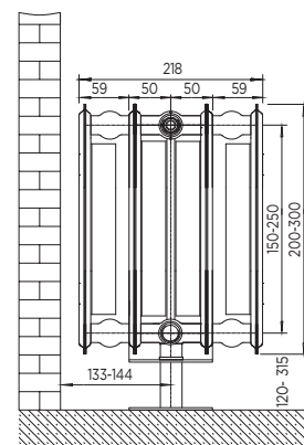
QS Quadruple Panel Single Convactor
